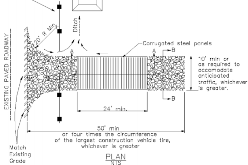
Sediment trapping device
